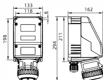
Wall type socket
