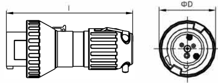
Plug
