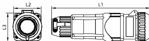
Coupler type socket
