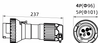
plug
