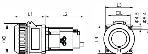
Panel type socket
