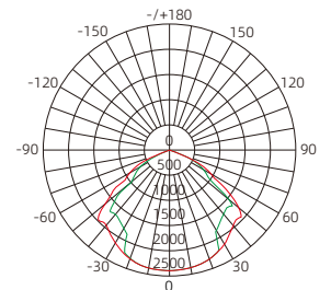
平均光束角 (50%) : 106.2度 The average beam angle (50%) : 106.2 Degree CZ0878/211 □-LED0060W 1
