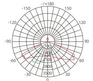
平均光束角 (50%) : 93.9度 The average beam angle (50%) : 93.9 Degree CZ0878/211 □-LED0060W SL
