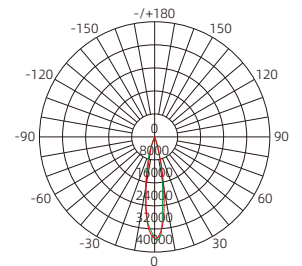
平均光束角 (50%) : 20.1度 The average beam angle (50%) : 20.1 Degree CZ0878/211 □-LED0060WNB
