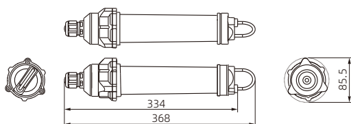
防爆设备灯 (不带钢丝网罩) Explosion-proof equipment light fittings (without steel mesh cover)
